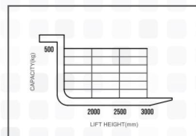
LOAD CHART
