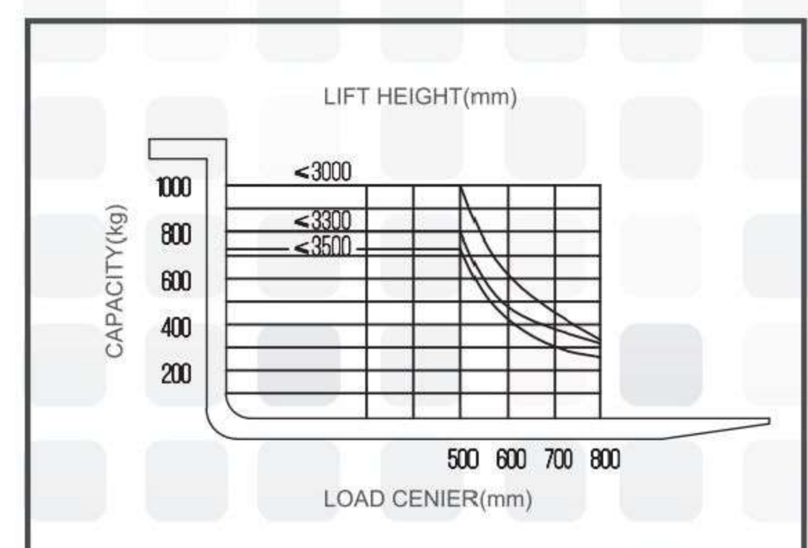
LOAD CHART
